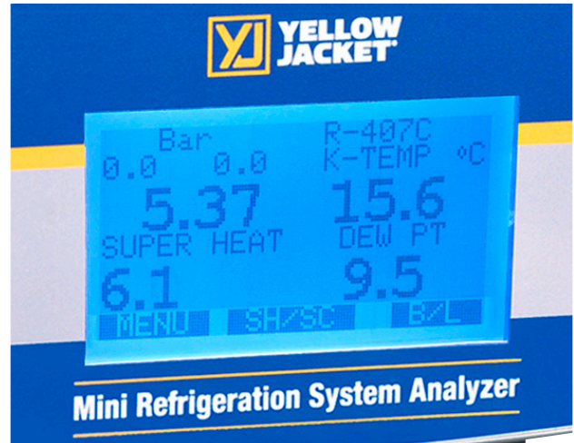
bar - Superheat
