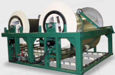
Coil Spool Assembly US Patent #7,673,915
